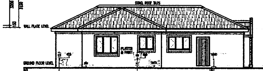
SOUTH ELEVATION
