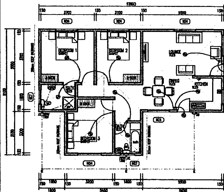
GROUND FLOOR PLAN Scale 1:100 (95.00 Sqm)
