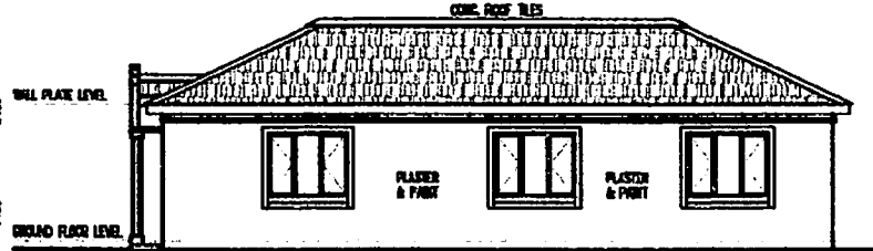
NORTH ELEVATION
