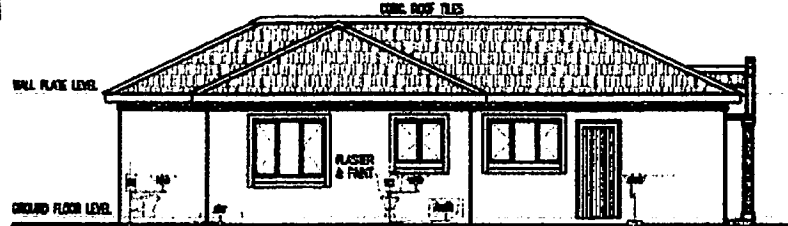
SOUTH ELEVATION
