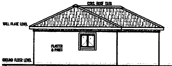
WEST ELEVATION
