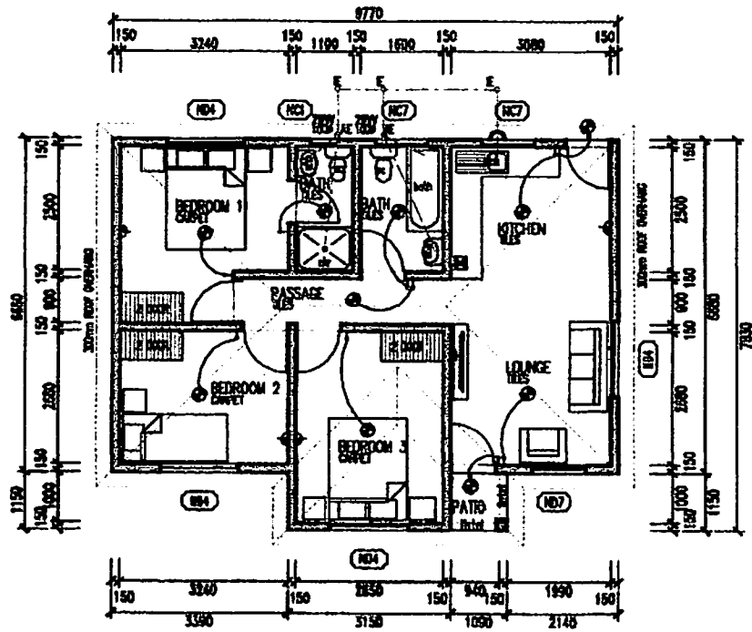
GROUND FLOOR PLAN Scale 1:100 (70.13 Sqm)
