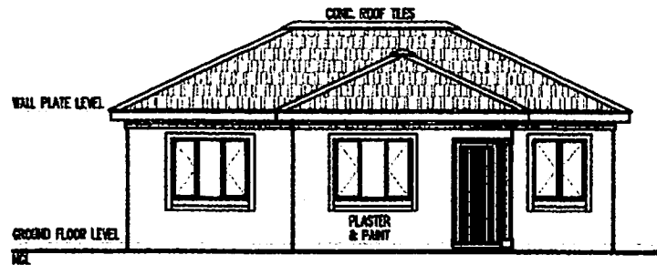
SOUTH ELEVATION
