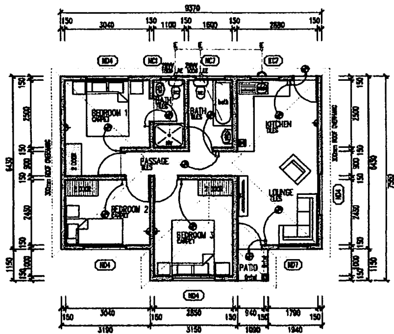
GROUND FLOOR PLAN Scale 1:100 (65.12 Sqm)
