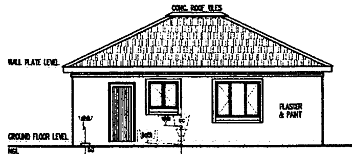
NORTH ELEVATION
