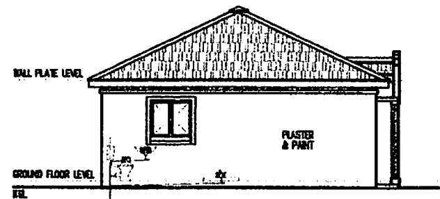
WEST ELEVATION
