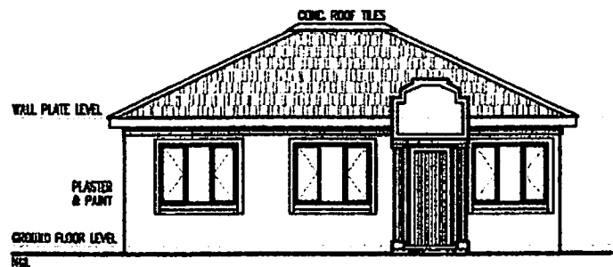
SOUTH ELEVATION
